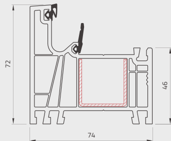
Telaio piano Flat frame
