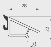
Trapezoidale Trapezoidal
